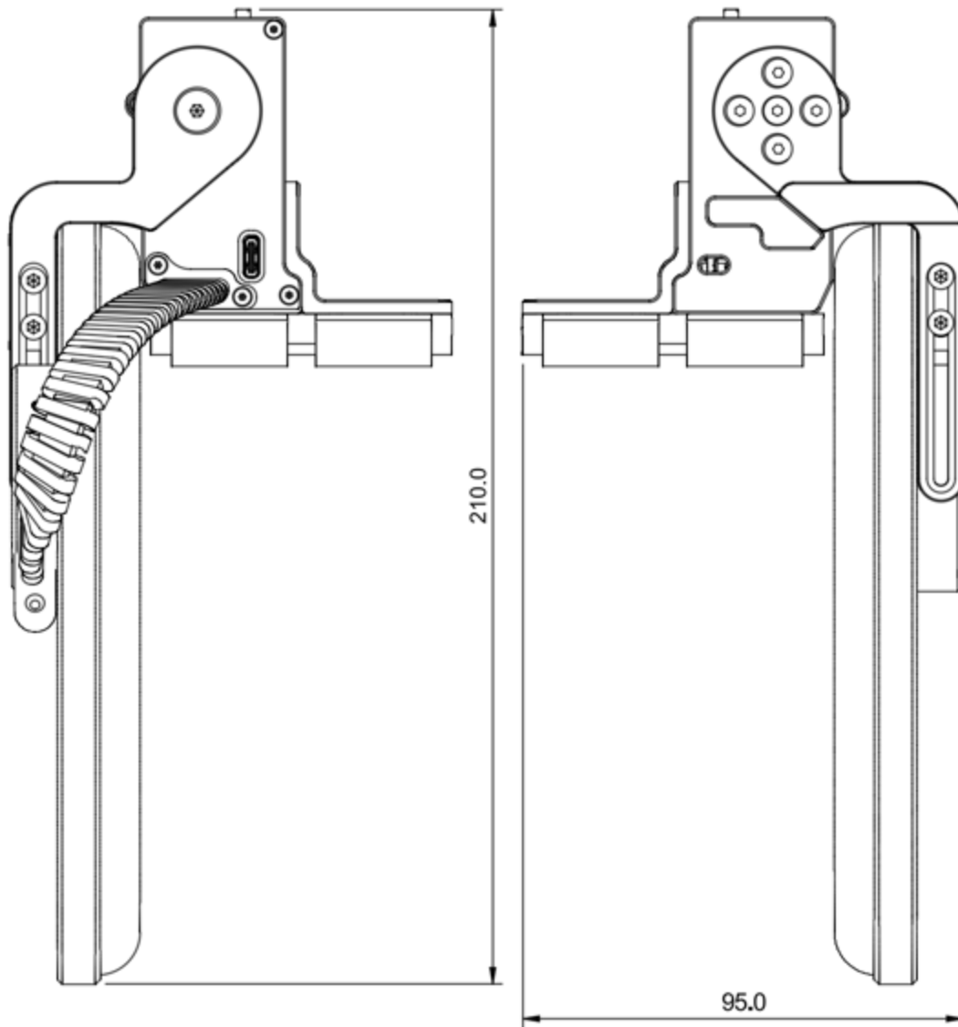
FM Neo 120 Side View
