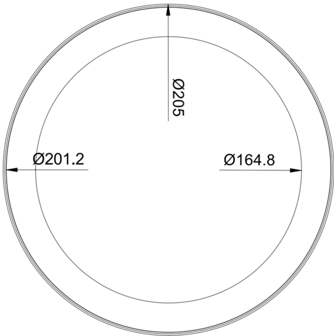
Cover ,LED and Silicone flange dimensions FM Neo 160
