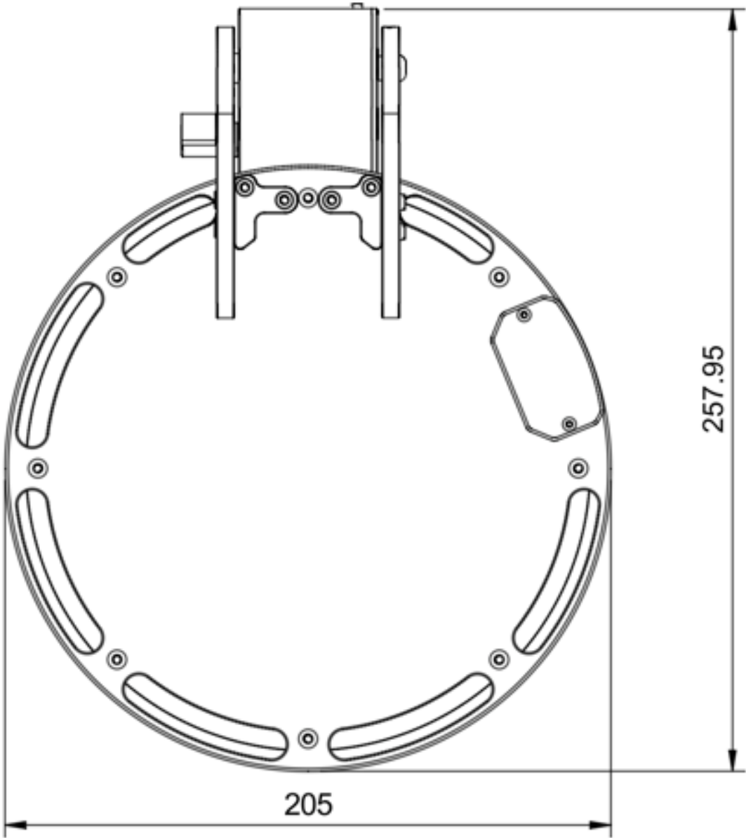
FM Neo 160 Front Side View
