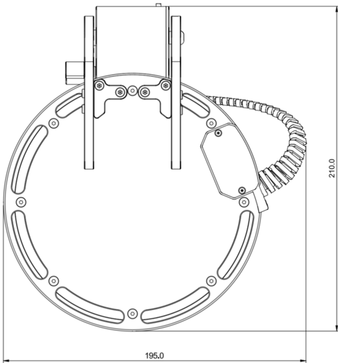
Front side FM Neo 120
