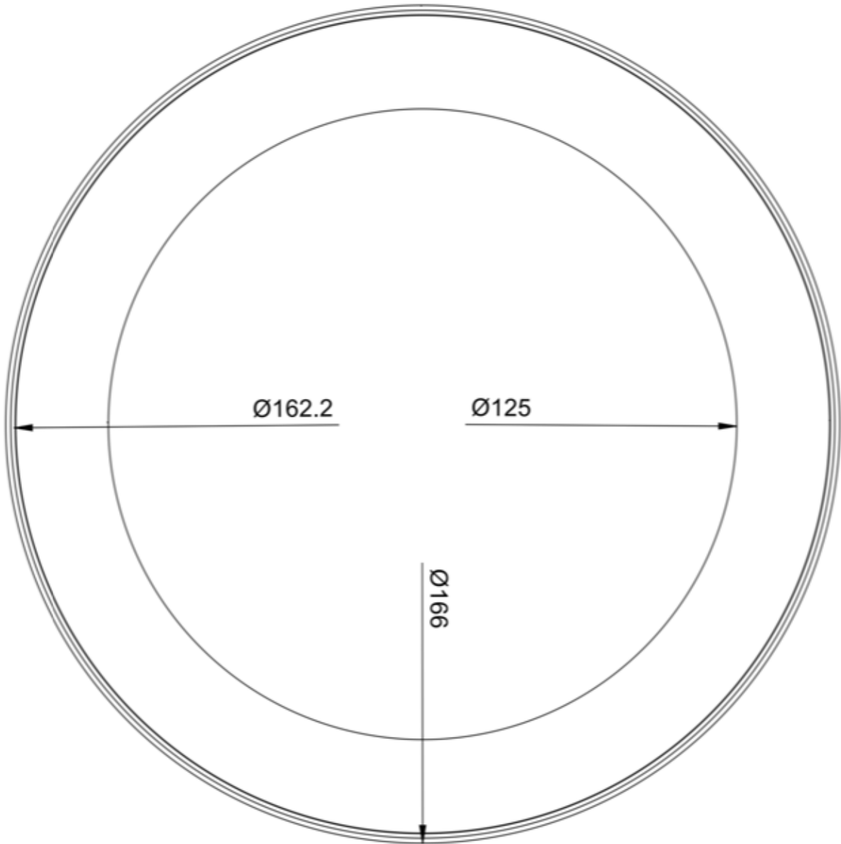
Cover ,LED and Silicone flange dimensions FM Neo 120
